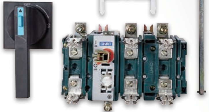
Components of the Fused-Switch Disconnecter
